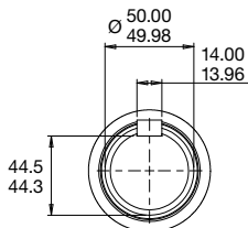
SHAFT END DETAIL
