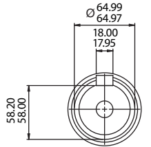
SHAFT END DETAIL
